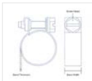
W1 - Zinc Plated Mild Steel Band, Screw & Nut W4 - Stainless Steel Band, Screw & Nut
